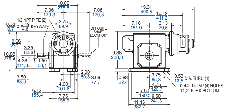
“B” Mounting (photo) 6AM-22A-GB40 / *6AM-22A-GF40 (standard shaft) / (opposite shaft) inches / mm
