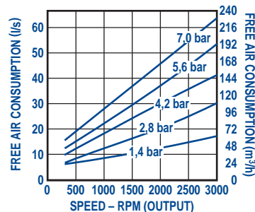
Air Consumption vs. Speed
